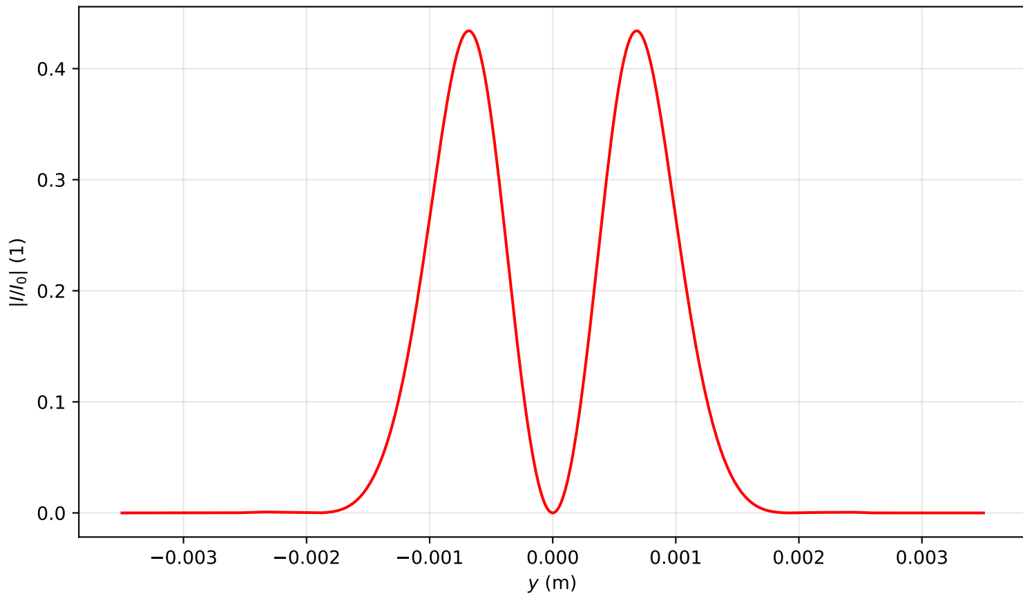
Intensity profile I(x = 0, y, z = 2.070)/I_0 , P_{in}=2.0P_{cr} , artificial time
